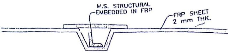
DETAIL 'A' - FRP DOME
