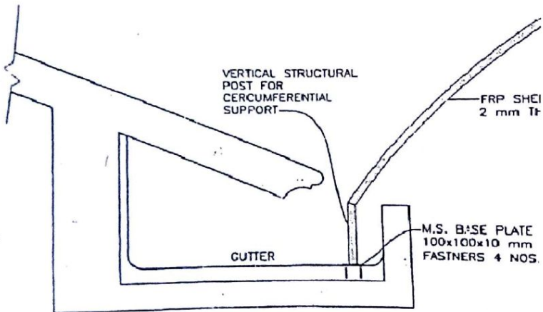
DETAIL 'B' - FRP DOME
